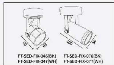
DIMENSION (mm)
