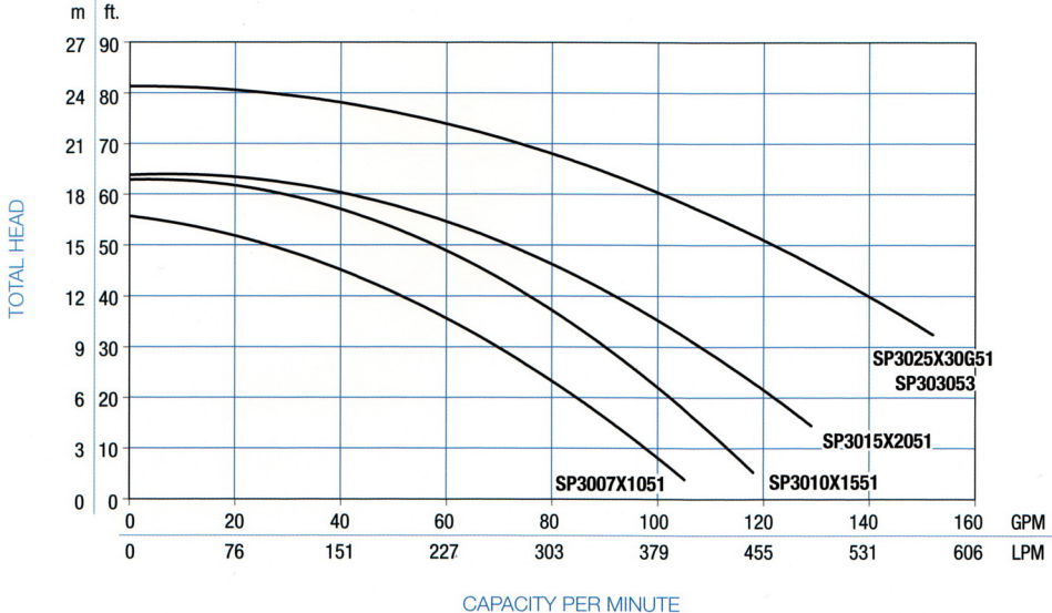
SUPER II PUMP FLOW VS. TOTAL HEAD
