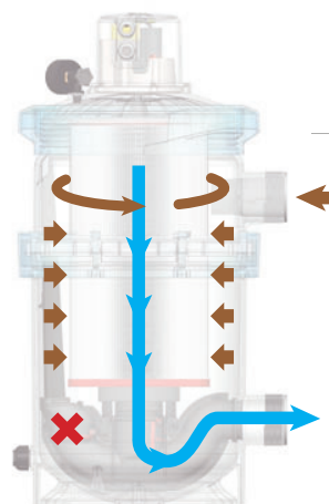
Water flow during filtration
