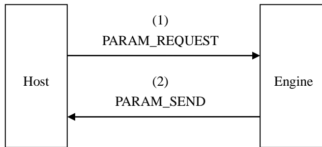
Figure 4-2 Host queries scanner's parameter
