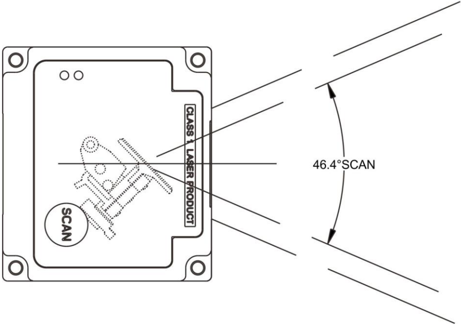
Figure 2-4 Scan angle
