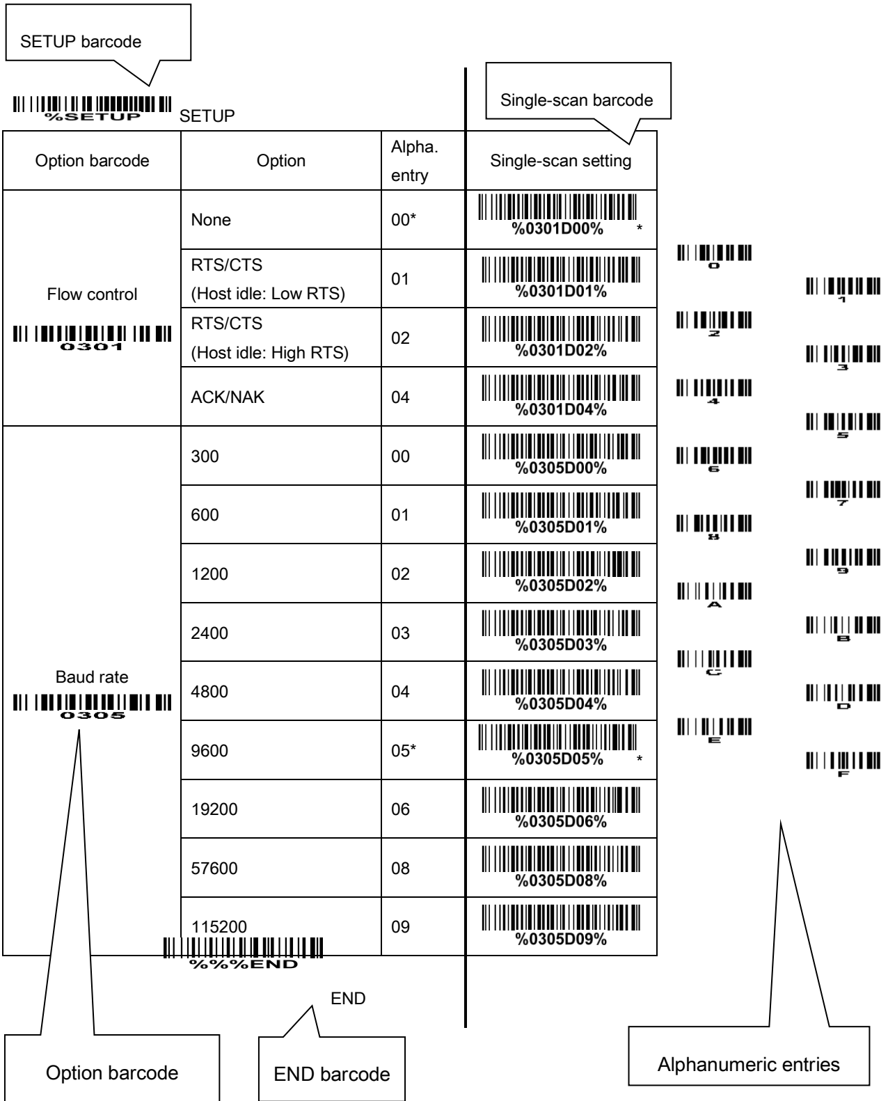
Figure 3-2 Set Flow control to be none
