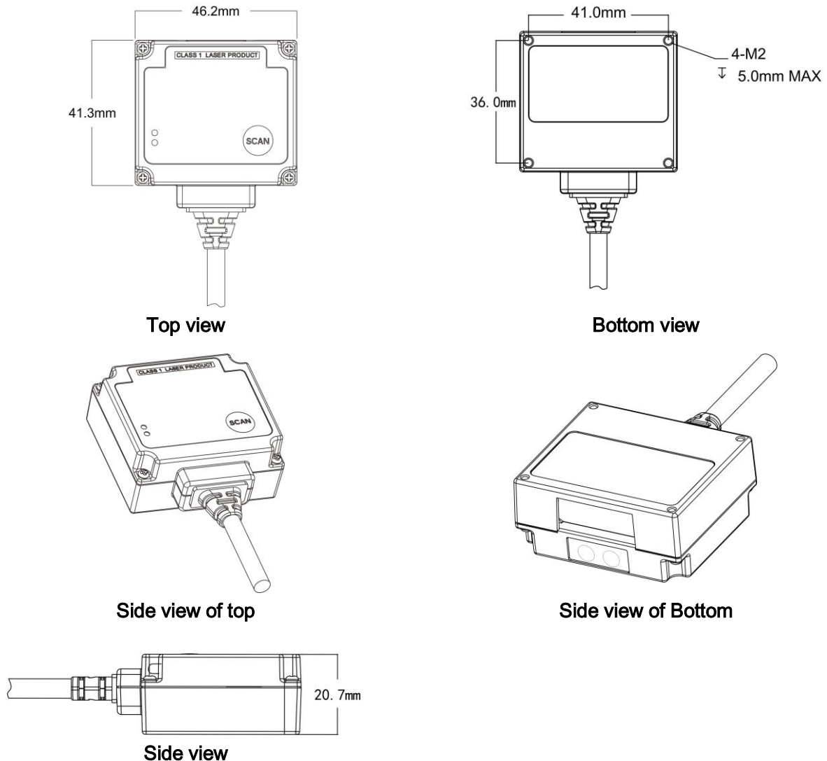
Figure 2-1 Mounting diagram
