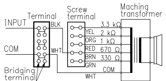
Wiring Diagram
