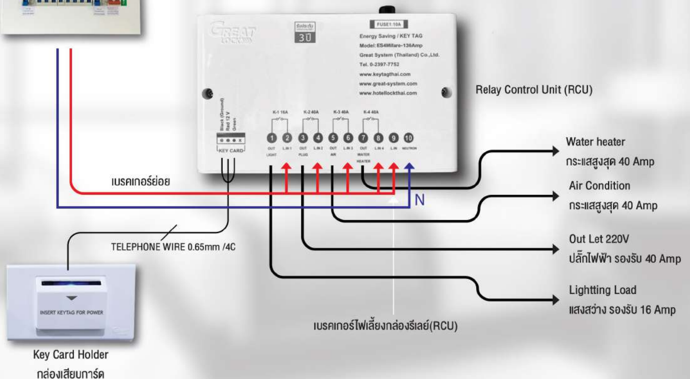
Consumer Unit Main 220V 50Hz.
