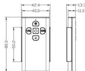
LEDSS-8040R
