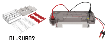
DL-SUB02 Multi-functional horizontal electrophoresis tank
