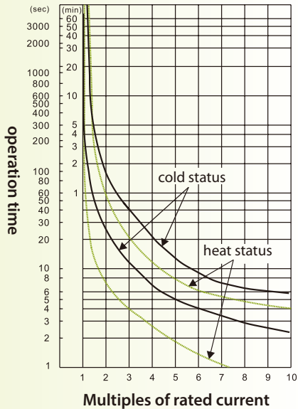
TH-P18ES – above 9A tripping characteristic curve
