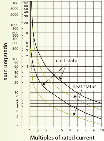
TH-P60ES TA tripping characteristic curve
