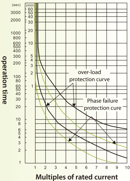
TH-P12ES PP tripping characteristic curve
