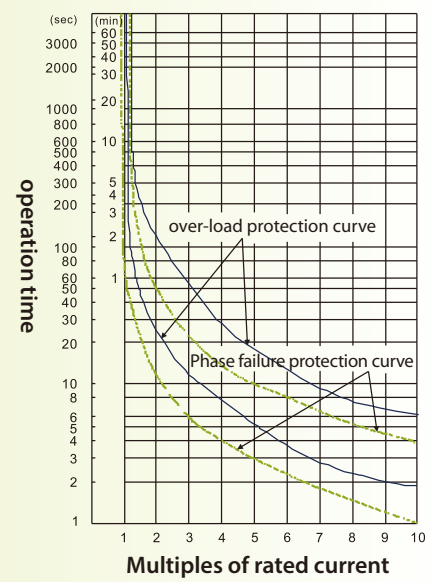
TH-P20ES TAPP tripping characteristic curve
