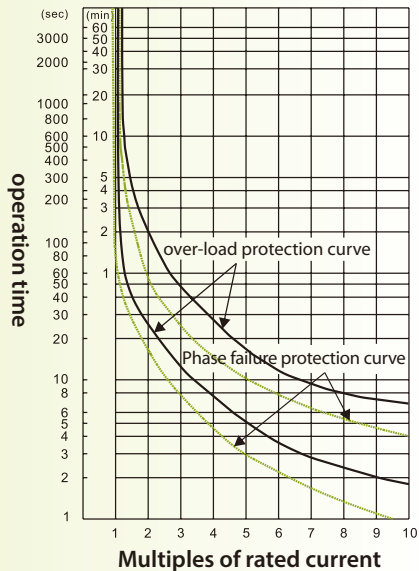
TH-P12ES TAPP tripping characteristic curve
