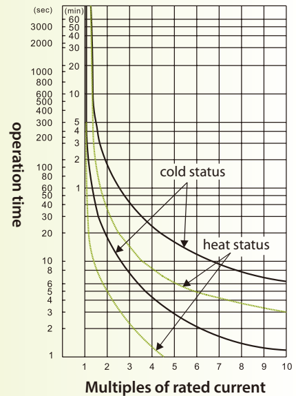
TH-P20ES – below 6.5A tripping characteristic curve
