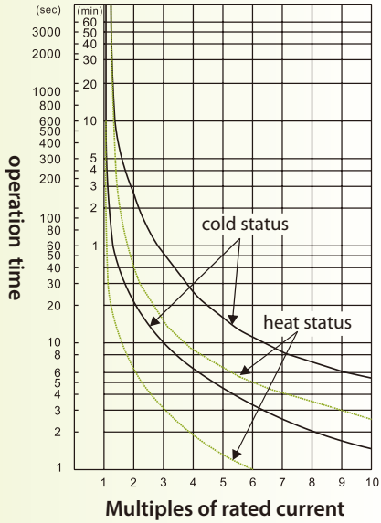
TH-P12ES tripping characteristic curve
