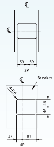
Panel cut
