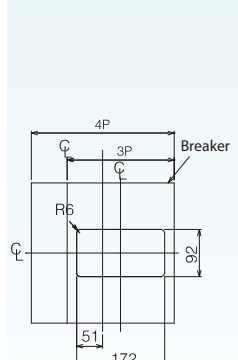
Panel cut
