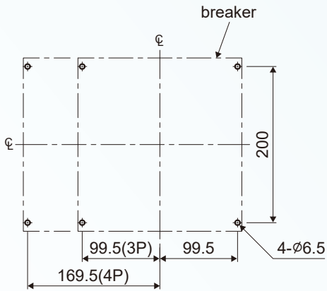
Panel drilling
