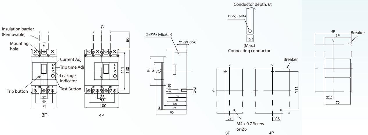
Panel cut
