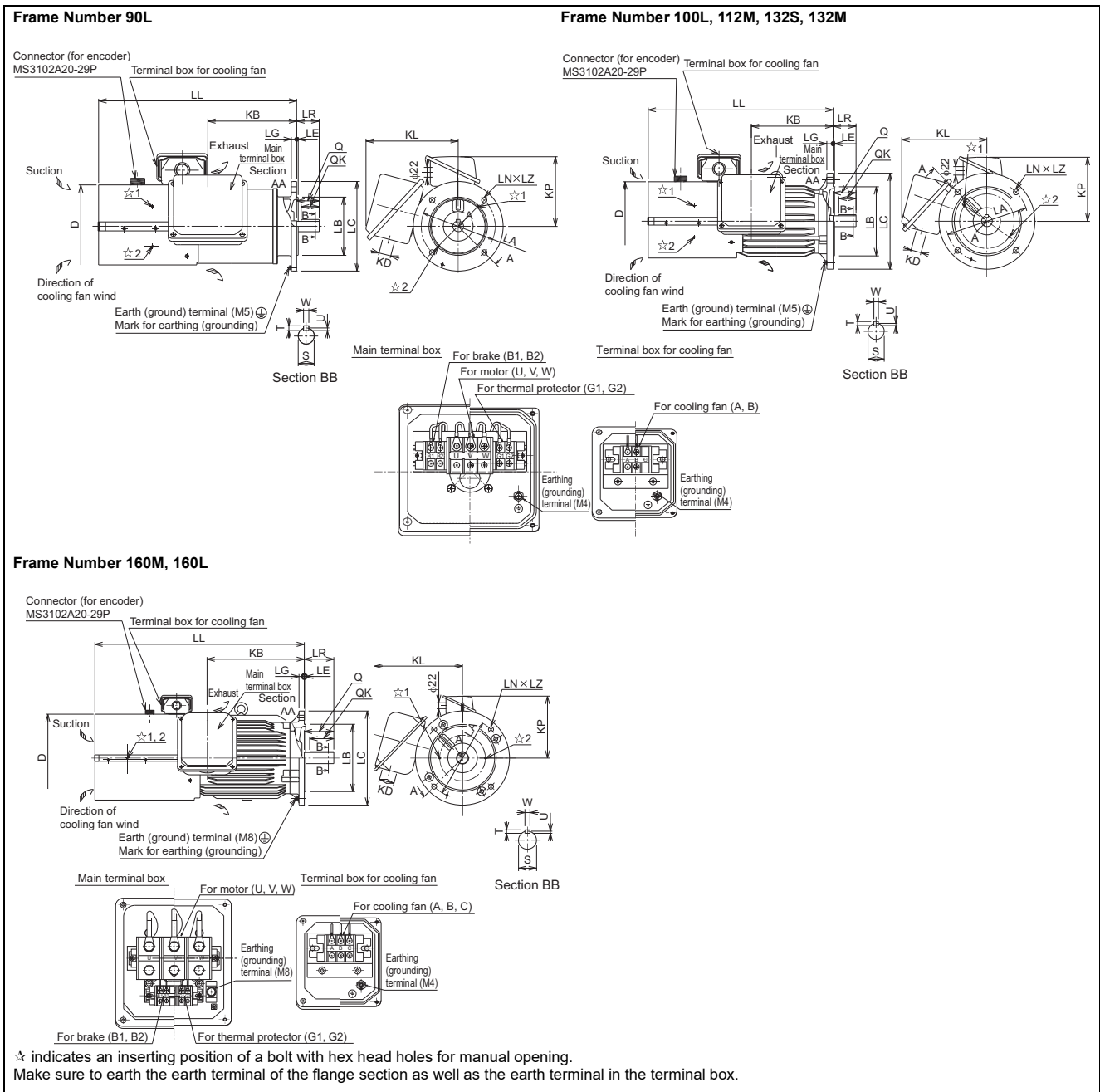
• Dimensions table (Unit: mm)
