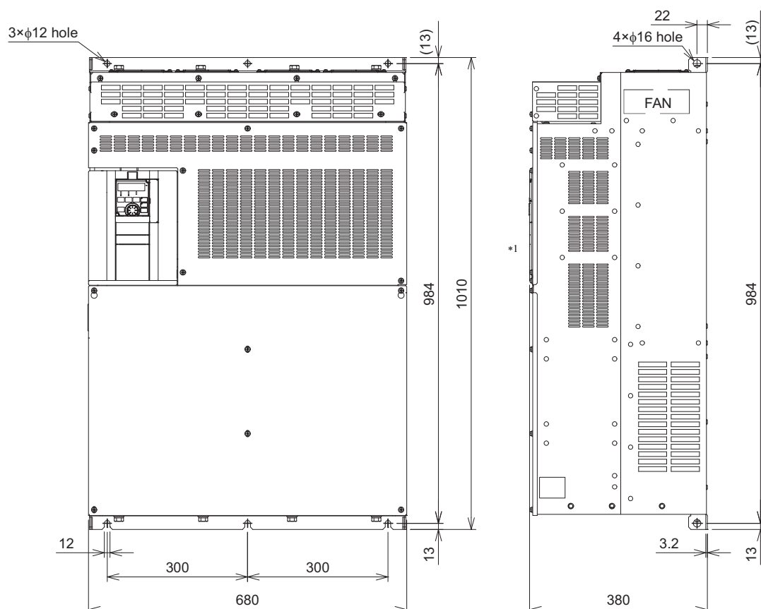
FR-A840-05470(220K), 06100(250K), 06830(280K)(-E)(-GF)(-GN)(-F)
