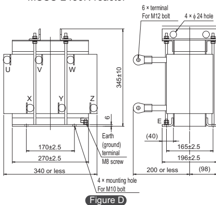
MSSU-2450N reactor
