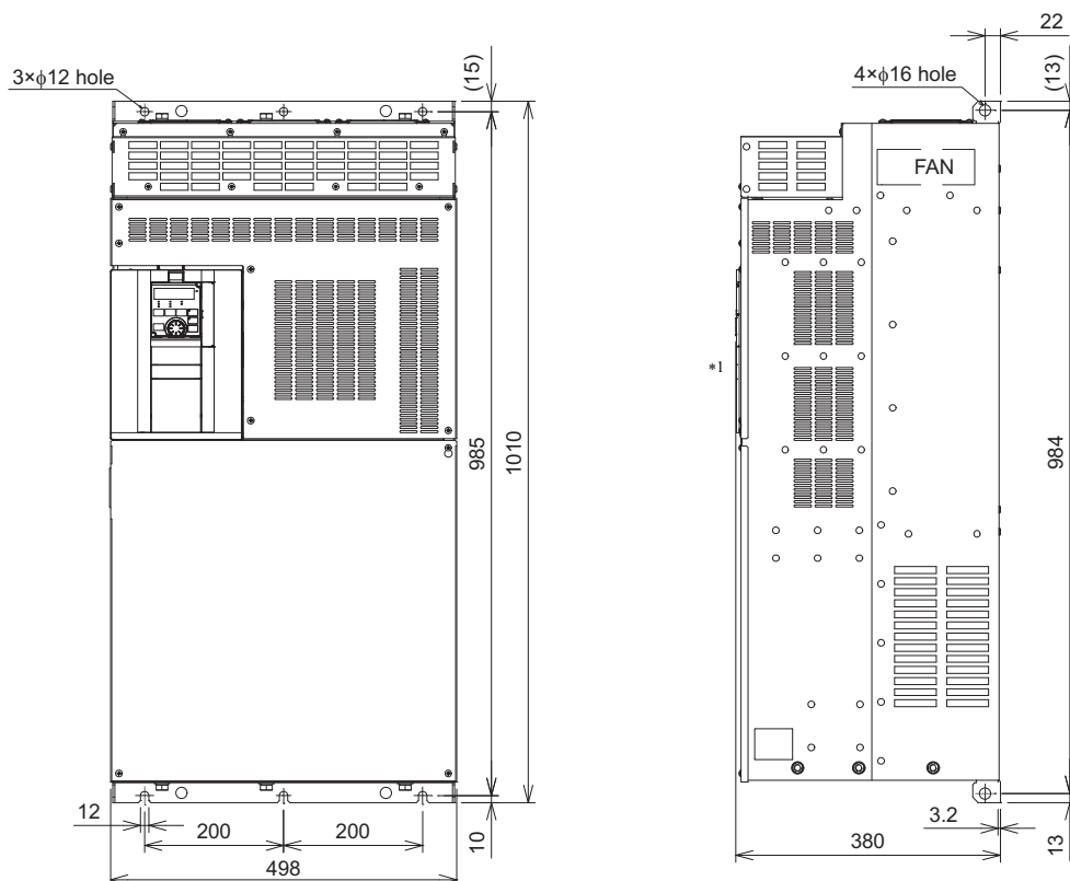
FR-A840-04320(160K), 04810(185K)(-E)(-GF)(-GN)(-F)
