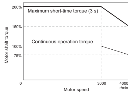
[Operation torque characteristics]
