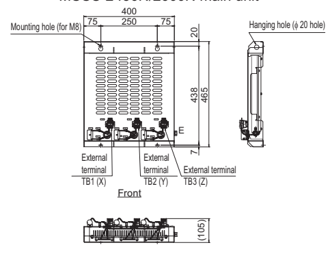
MSSU-2450N/2600N main unit
