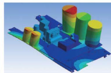
3D-vibration analysis
