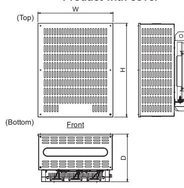
MSSU-2150/2220/2340 Product with cover
