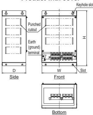
MSSU-2010C to 2110C Product with cover
