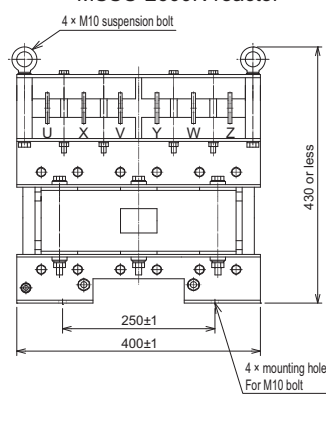
MSSU-2600N reactor
