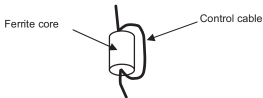
Example of installing ferrite cores
