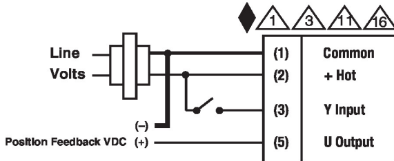
Floating Point AC 24 V Transformer (AC Only)
