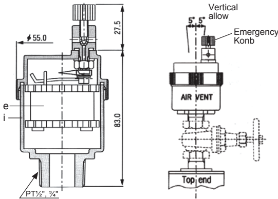
Float type by bubble crush method for water
