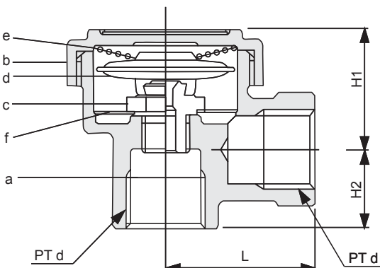
Capsule type for steam
