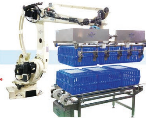
• ROBOTIC PALLETIZER FOR BIRD CAGE (STACKING)
