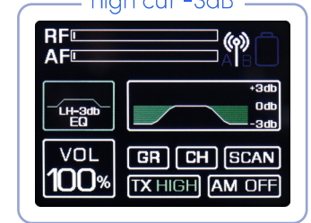
low cut -3dB high cut -3dB
