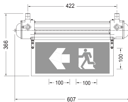
Body 2 (4 cable entries)
