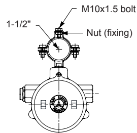
Pendant mount (for chain)
