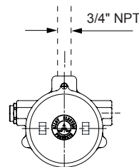
Pendant mount (for pipe)
