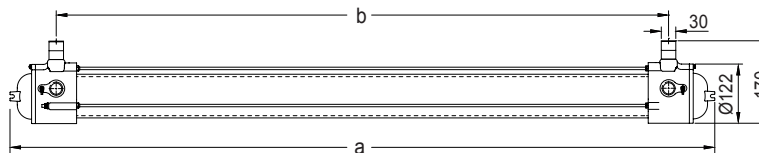
Body 2 (4 cable entries)
