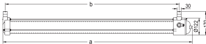
Body 2 (4 cable entries)
