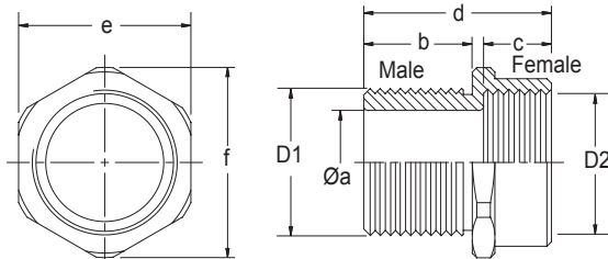
Thread type: NPT male to NPT female
