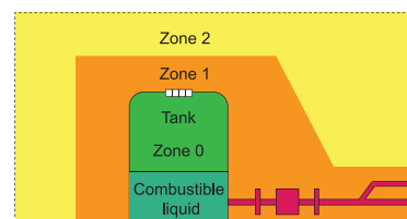
Example of zones classification for flammable liquid and vapor
