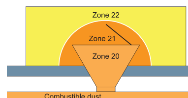
Example of zones for combustible dust
