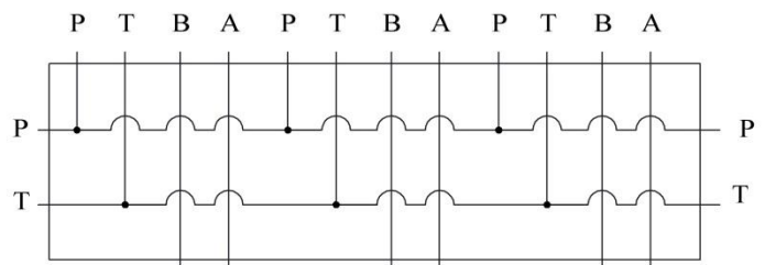
Oil circuit
